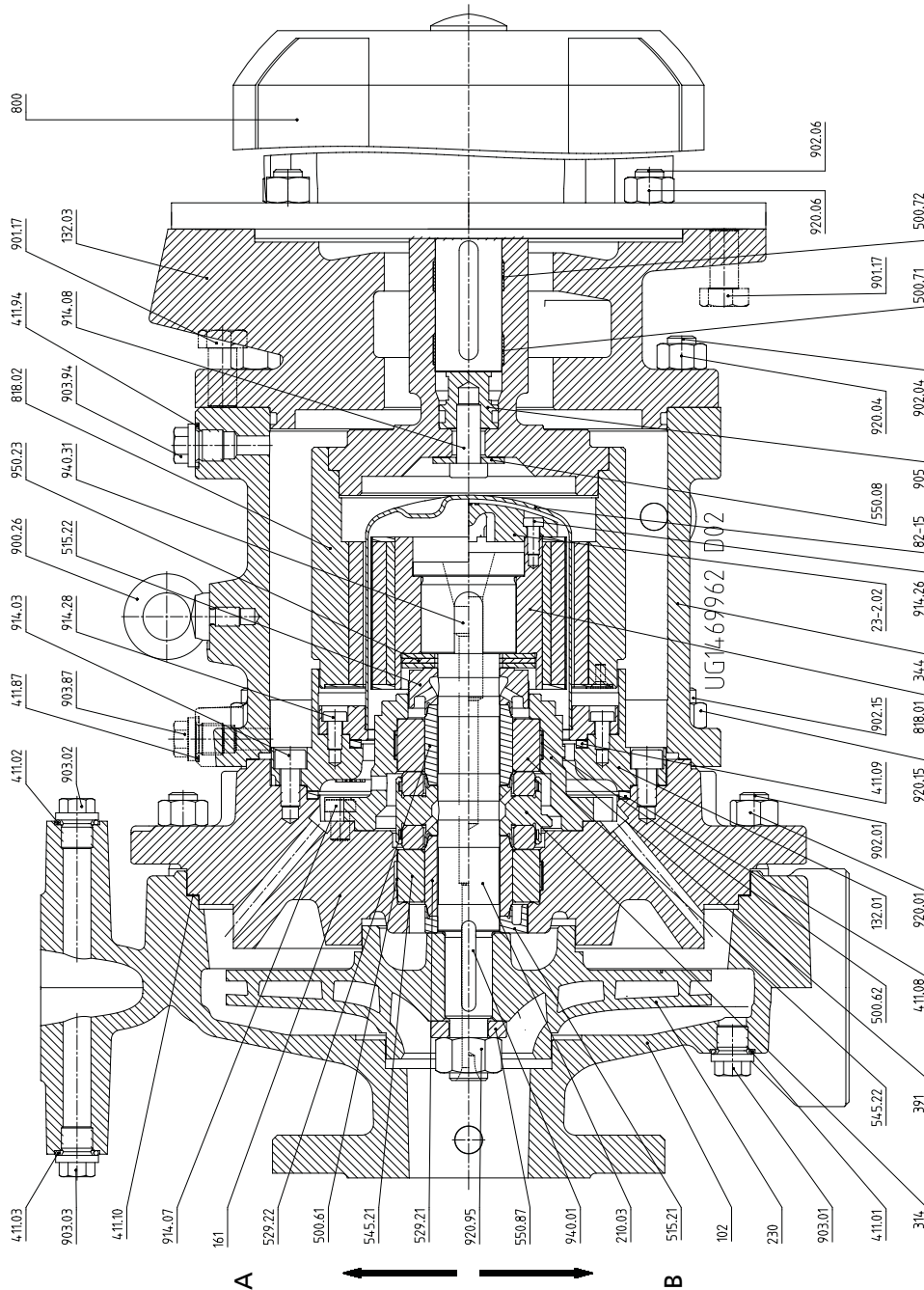
Fig. 15: General assembly drawing of model with bolted cover, with intermediate piece
