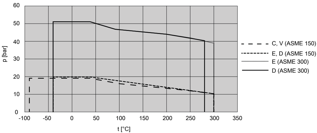
Fig. 2: Pressure limits and temperature limits of ASME flanges 5)
