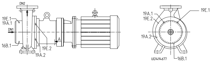
Fig. 13: Connections for heating 18)
