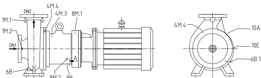
Fig. 12: Connections for dead-end configuration operating mode
