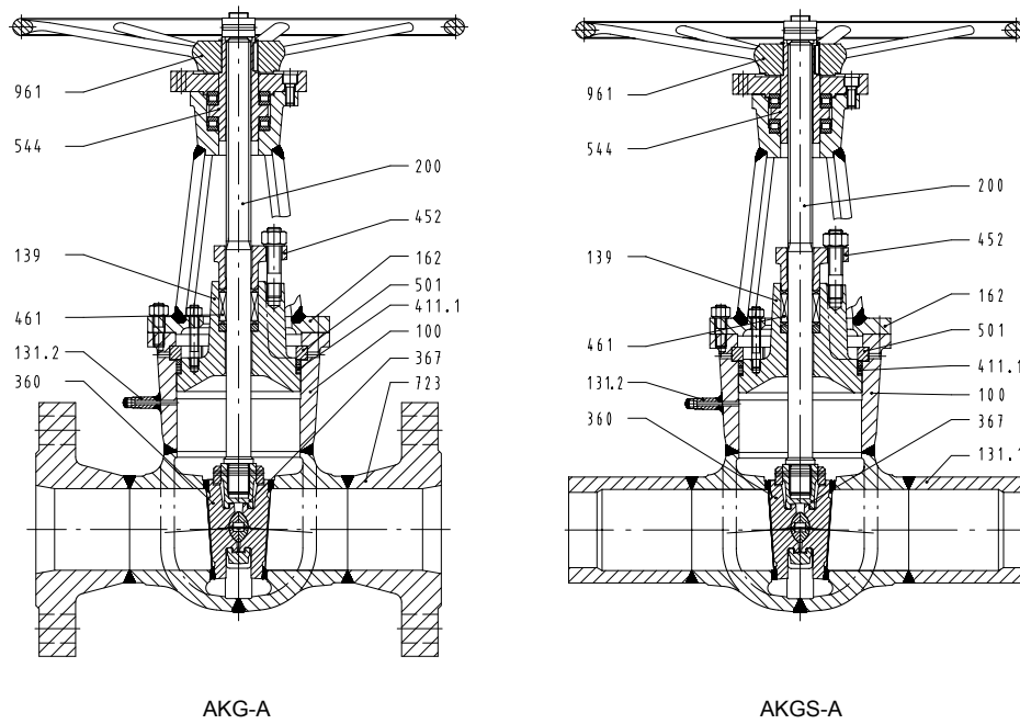
Fig. 1: Sectional drawings
